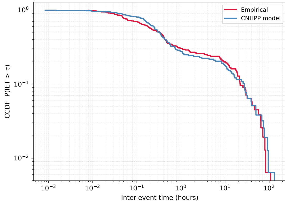
User 1357872899 - Empirical vs CNHPP model
